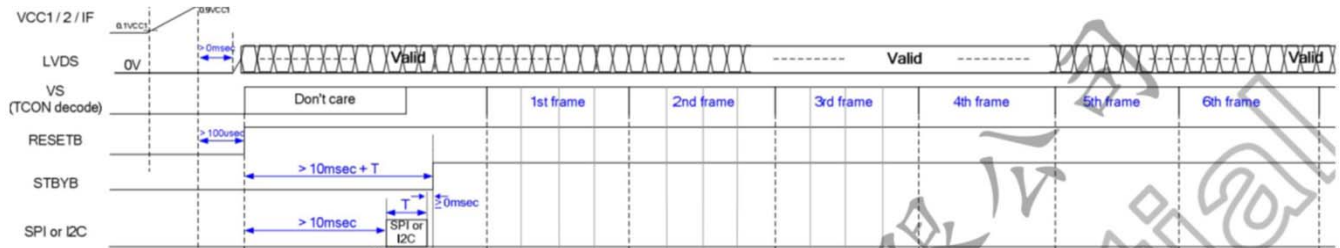
Power-on Sequence
