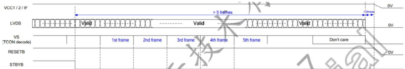
Power-off Sequence
